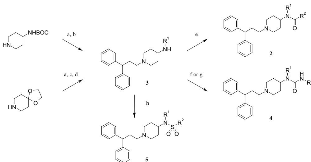
Scheme 1. Reagents and conditions: (a) 3,3-diphenylpropyl bromide, K_2CO_3 , tBu_4NI (0.1 equiv), MeCN, reflux, 5 h; (b) ( R^1 = Me ) LiAlH_4 , THF, reflux, 5 h; (c) 6 M HCl, reflux, 3 h; (d) R^1NH_2 , NaBH_3CN , AcOH, MeOH, rt; (e) R^2CO_2H , DIPCDI, HOBT (0.1 equiv), DMF/DCM, rt; (f) R^2NCO , DCM, rt; (g) R^2CO_2H , DPPA, Et_3N , THF, 0 °C then toluene, 100 °C then 3, EtOAc, rt; (h) R^2SO_2Cl , (iPr)_2NEt , MeCN/pyridine.
